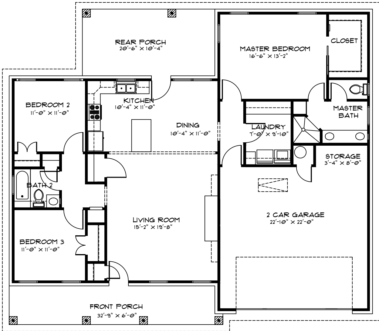
FLOOR PLAN
