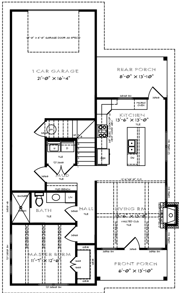
FIRST FLOOR FLOOR PLAN
