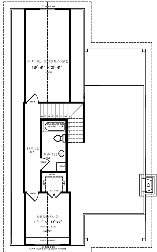
SECOND FLOOR FLOOR PLAN
